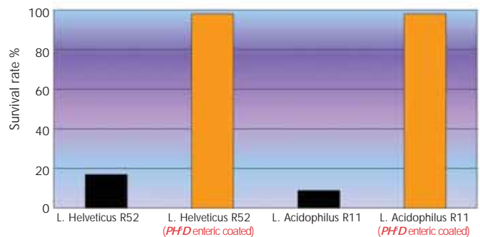
Survival rate of probiotic bacteria with & without PH F D protection (30 min at PH 2)
